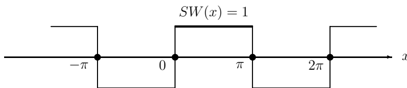
Figure 4.1: The odd square wave with SW(x + 2\pi) = SW(x) = \{1 \text{ or } 0 \text{ or } -1\} .
