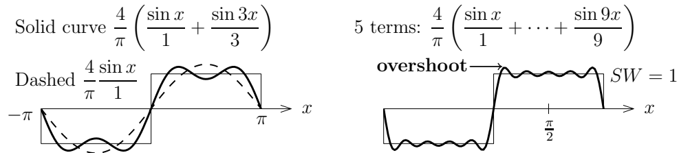
Figure 4.2: Gibbs phenomenon: Partial sums \sum_1^N b_n \sin nx overshoot near jumps.
